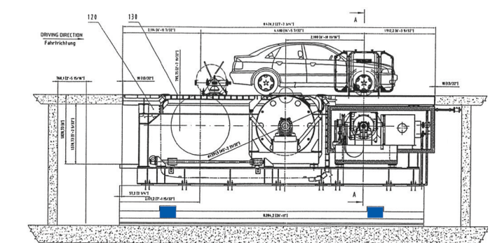
Chassis dynamometer on a vibration-isolated foundation
