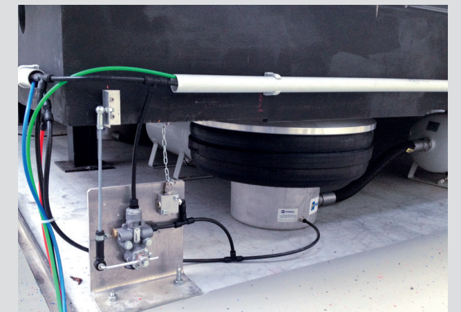
SAF Holland test bench
