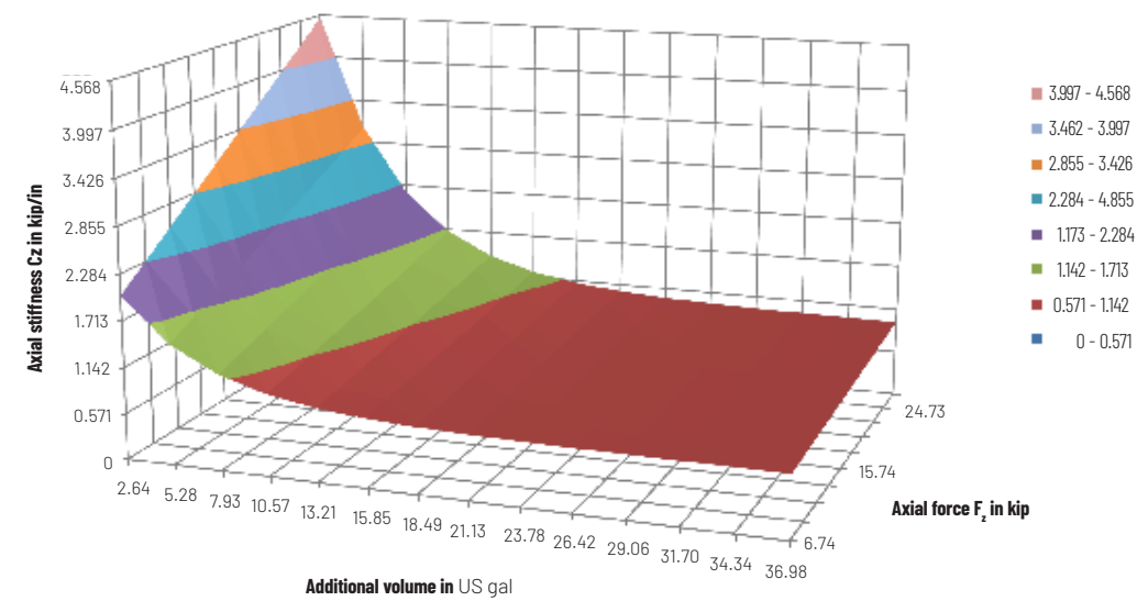
RLA260: Axial stiffness C_z over additional volume and axial force
