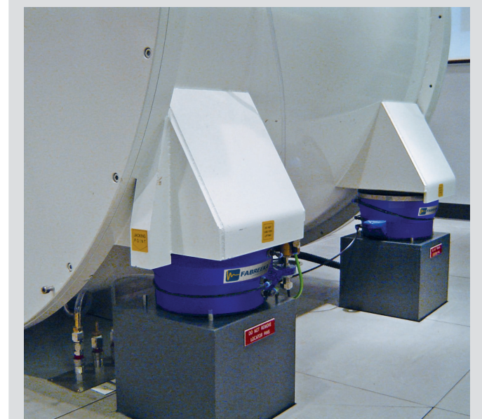
600 MHz NMR on PAL18 gimbal air springs
