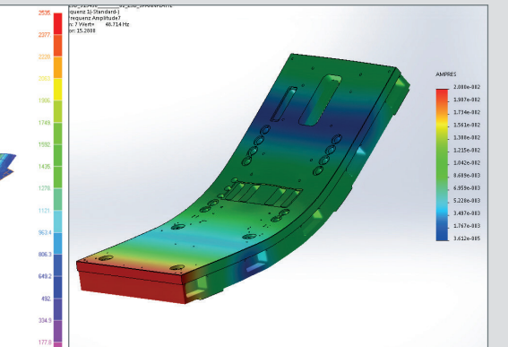
Fig. 13: First bending frequency from the G625 measuring plate
