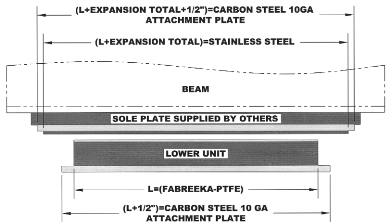
SIDE ELEVATION
