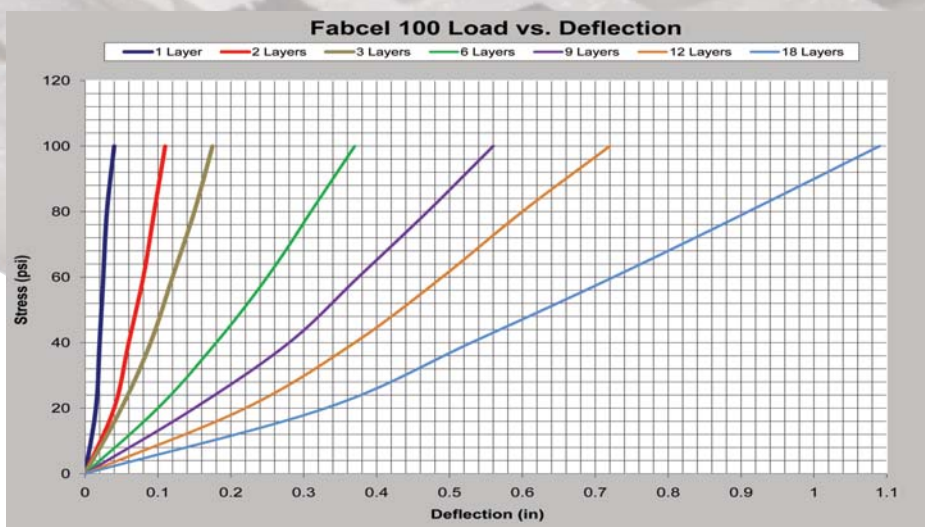
Figure 8 Load Deflection
