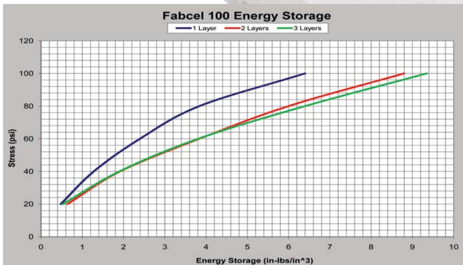
Figure 9 Energy Storage
